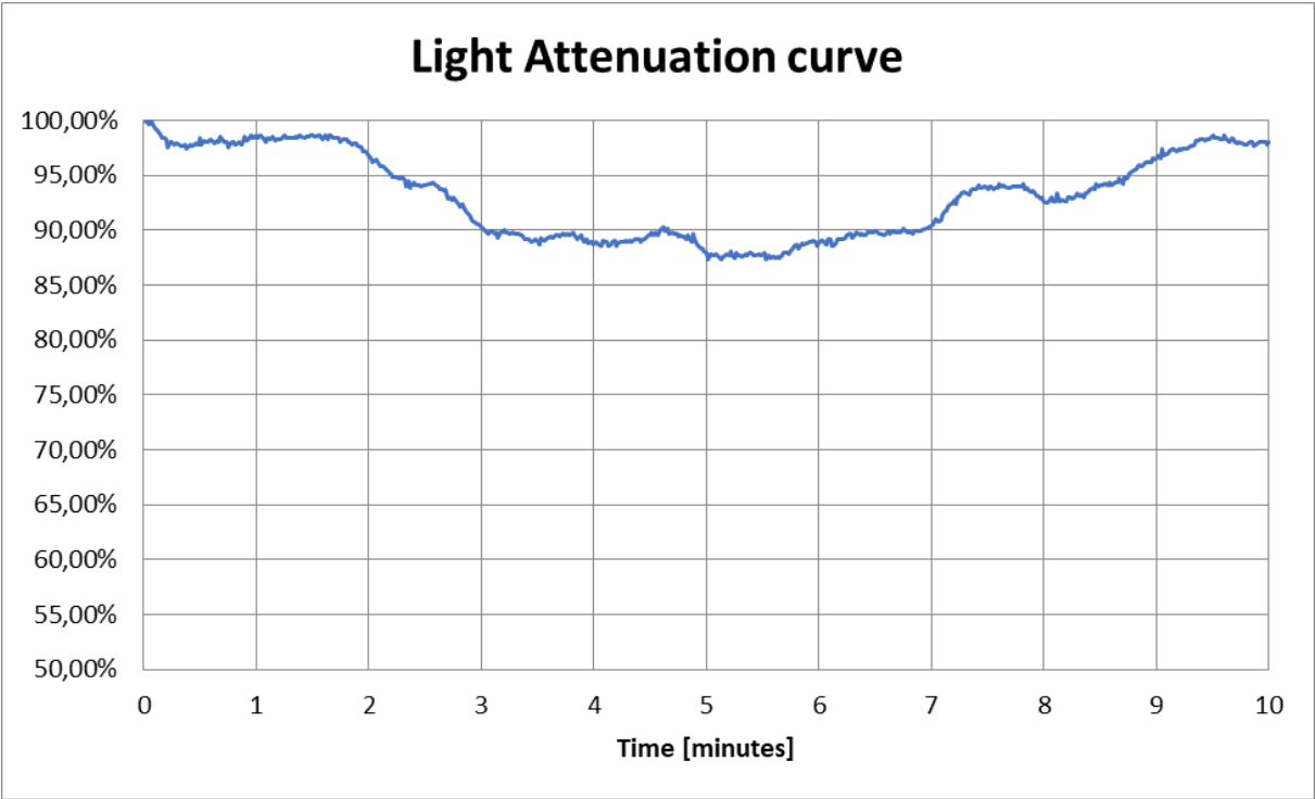
Light attenuation curve - test specimen No. 1:
