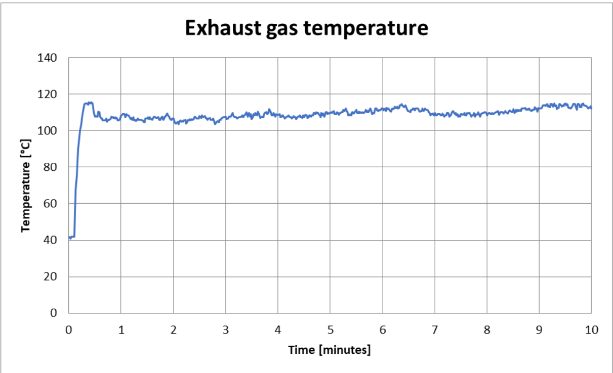
Smoke temperature curve - test specimen No. 1:
